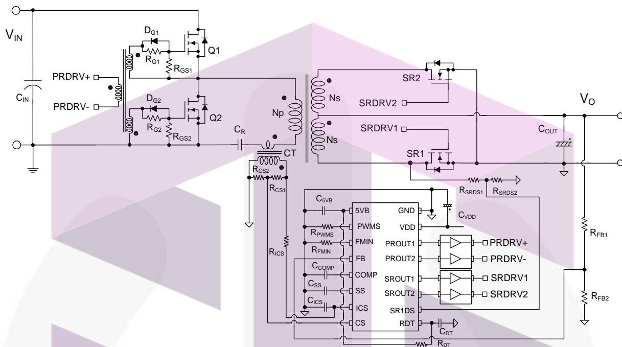
Figure 2. Typical Application
